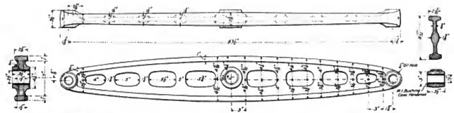
Figs. 1659-1663. Cast-Steel Equalizer. Eight-Wheel (4-4-0) Locomotive. Chicago & Alton.
